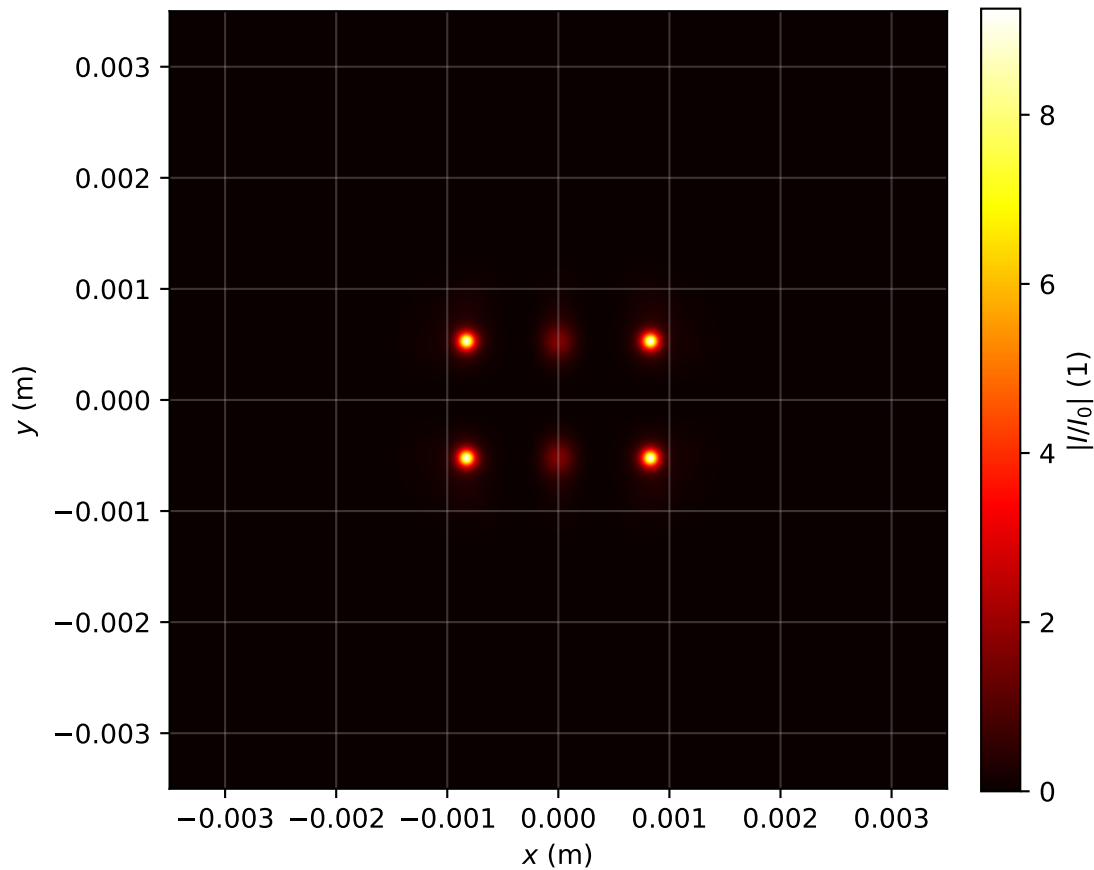
Intensity profile I(x, y, z = 0.478)/I_0 , P_{in}=8.0P_{cr} , artificial time
